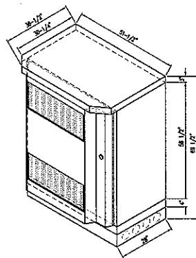
TYP. BTS DETAIL NOT TO SCALE
